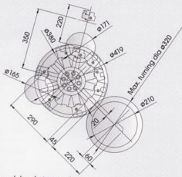
12-Station block turret
