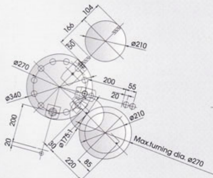
VDI 30 12-Station power turret
