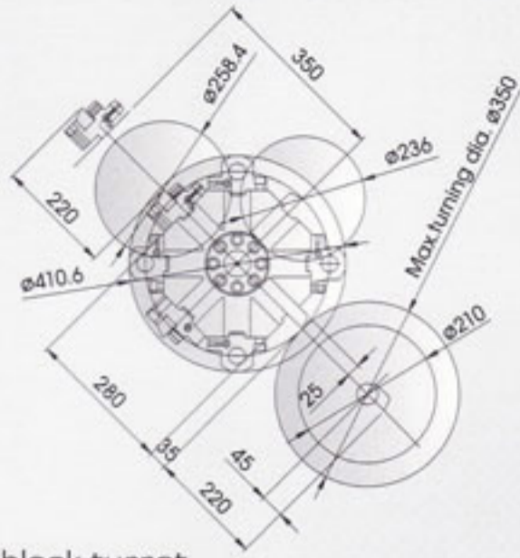
8-Station block turret
