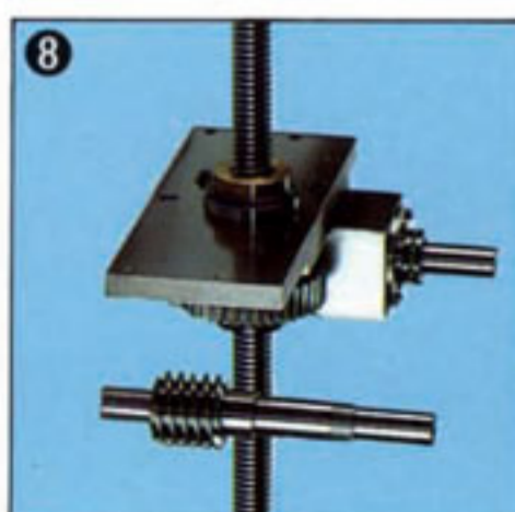
• Hardened & ground vertical lead-screw and transmission gears.
